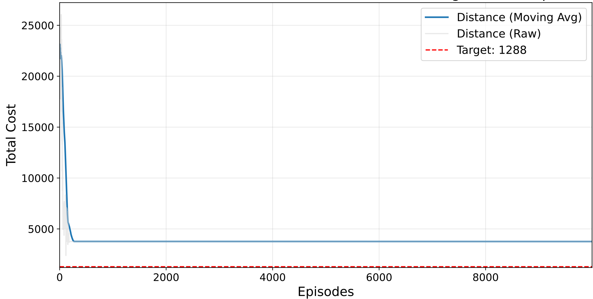
Final HYPERBAND GP Masked AutoRL-SOP Training - ESC47.sop
